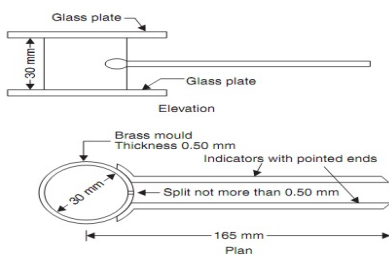
Fig. 2: Schematic of Le-Chateliers Apparatus
