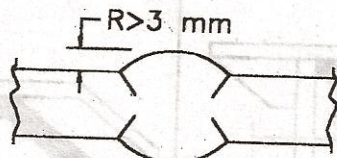
EXCESSIVE CONVEXITY
