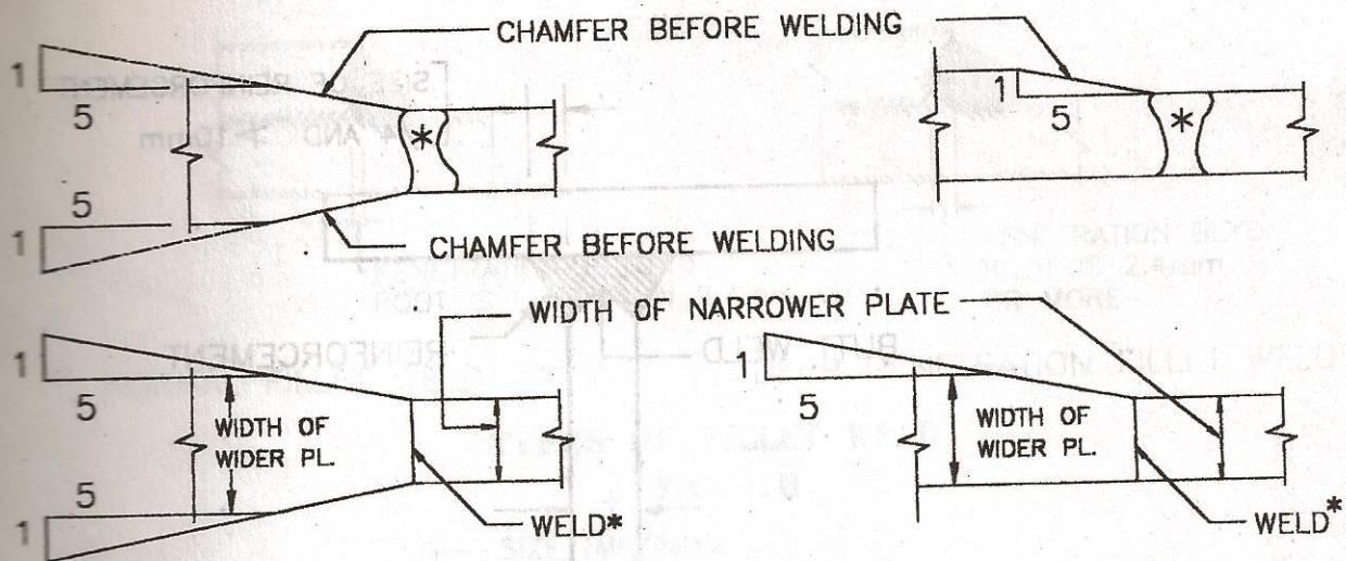
TRANSITION BY CHAMFERING THICKER OR WIDER PART
