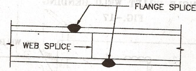
AVOIDING ACCUMULATION OF WELD JOINTS
