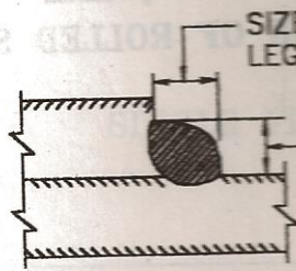
FILLETS OF UNEQUAL LEG LENGTH (NOT PERMITTED)
