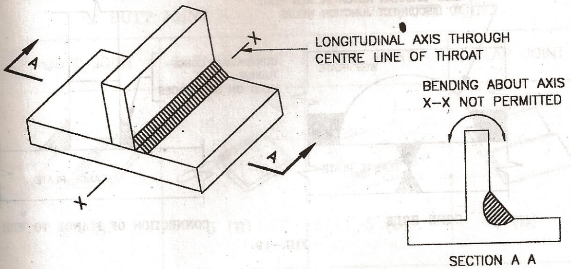
SINGLE FILLET WELD BENDING FIG.-17
