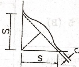
ACCEPTABLE FILLET WELD PROFILE FIG.-25
