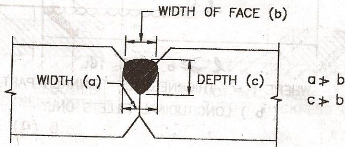
DIAGRAM OF WELD PASS IN BUTT WELD SHOWING DEPTH OF FUSION IN CROSS SECTION AND WIDTH OF FACE
