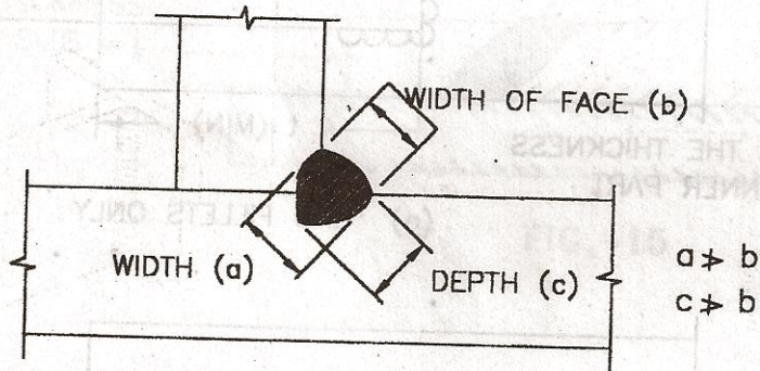
DIAGRAM OF WELD PASS IN FILLET WELD SHOWING DEPTH OF FUSION WIDTH IN CROSS SECTION AND WIDTH OF FACE
