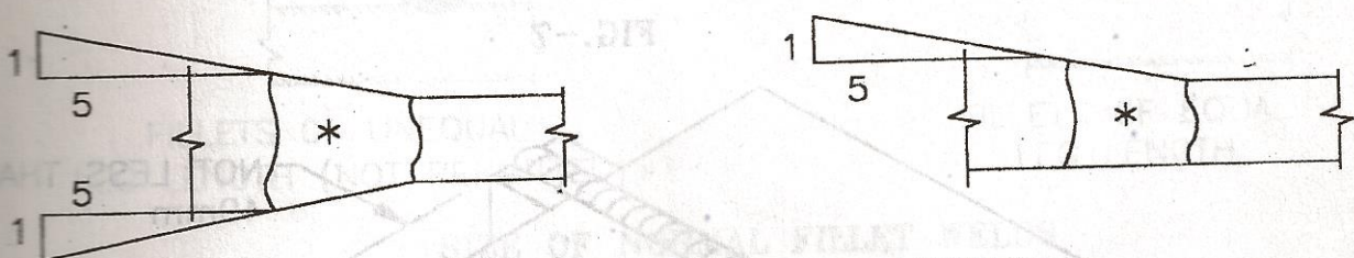
TRANSITION BY SLOPING WELD SURFACE
