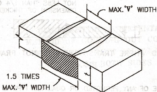
BUTT WELD END REINFORCEMENT
