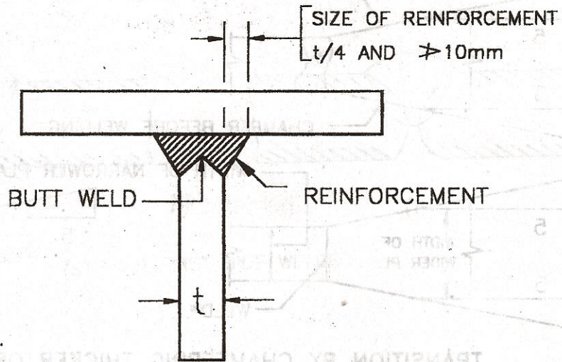
BUTT WELDED T JOINT
