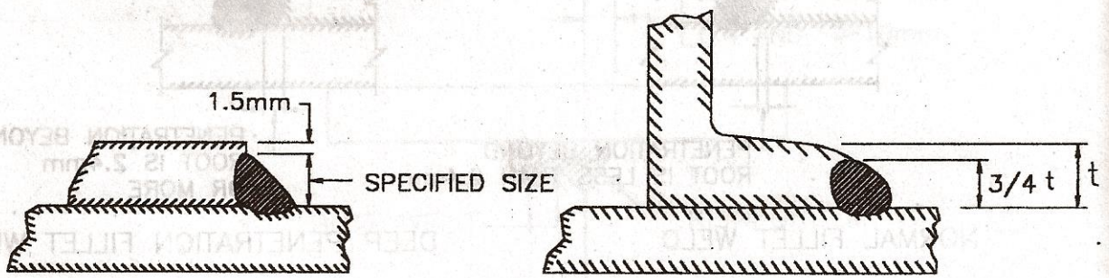
FILLET WELD APPLIED TO SQUARE EDGE OF PLATE OR ROUND TOE OF ROLLED SECTION
