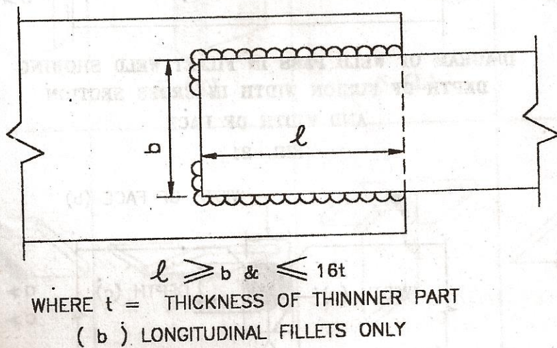
FILLET WELDS IN LAP JOINTS FIG.-18
