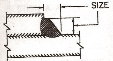
FILLETS OF EQUAL LEG LENGTH
