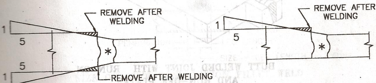
TRANSITION BY SLOPING WELD SURFACE AND CHAMFERING
