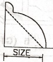
EXCESSIVE CONVEXITY
