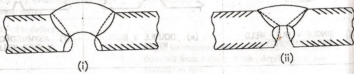
(b) BACK OF FIRST RUN GOUGED TO CLEAN METAL
