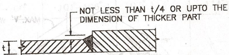
BUTT WELD WHERE TRANSITIONING IS NOT PRACTICABLE
