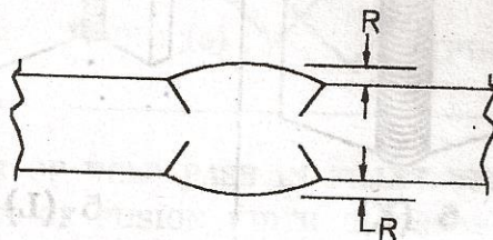
ACCEPTABLE BUTT WELD PROFILE FIG.-27
