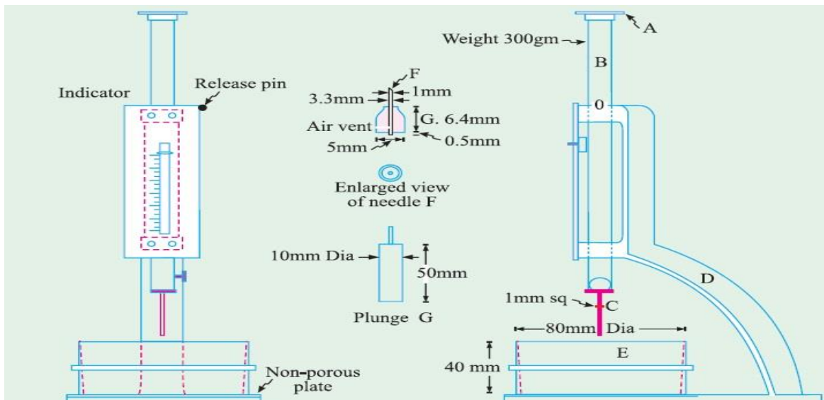
Fig. 4: Needles used in Vicat's Apparatus
